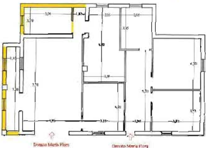
Post Operam Piano Seminterrato
