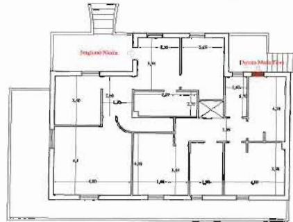
Post Operam Piano Terra
