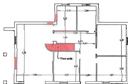
Post Operam Piano Seminterrato
