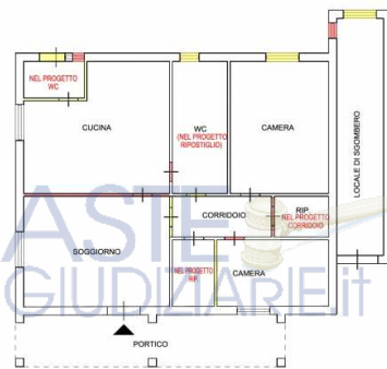
PIANO TERRA scala 1:100
